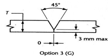
Figure 8 Plate test assembly for S classification for SMAW, GMAW, and GTAW processes
